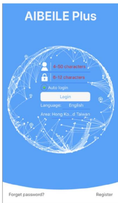
Login screen
